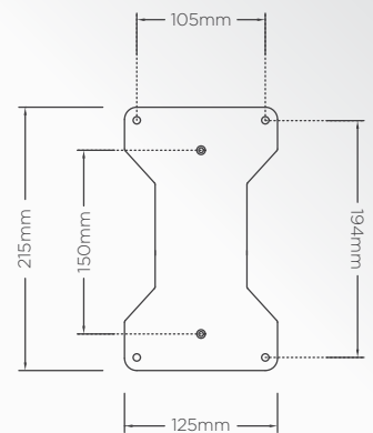
Mounting plate:
